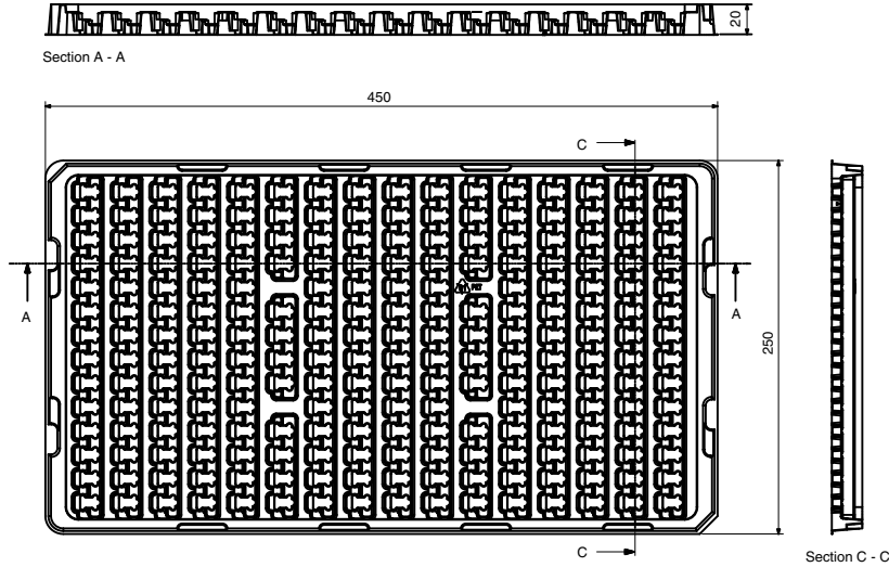
Drawing-No. 9.700-5307.01-1 Issue 1; 17.06.09 21799
